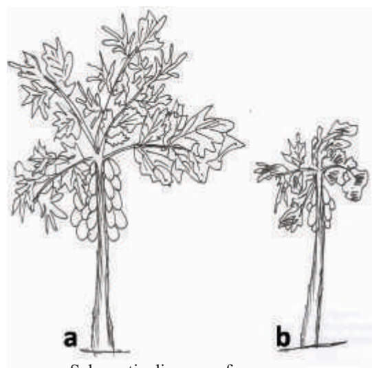
Schematic diagram of (a) virus-resistant transgenic and (b) susceptible papaya cultivar
